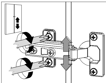
B. Vertical adjustment (Moving Door Up-Down) via slot in the mounting plate
