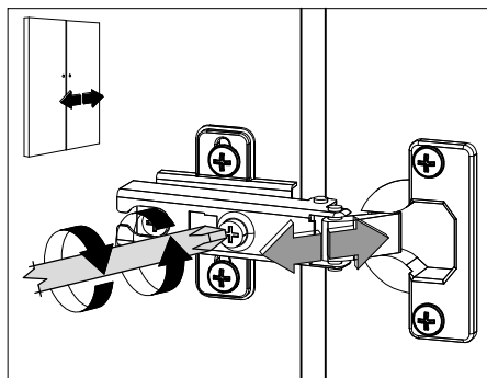
A. Lateral adjustment (Moving Door Left-Right) by screw adjusting
